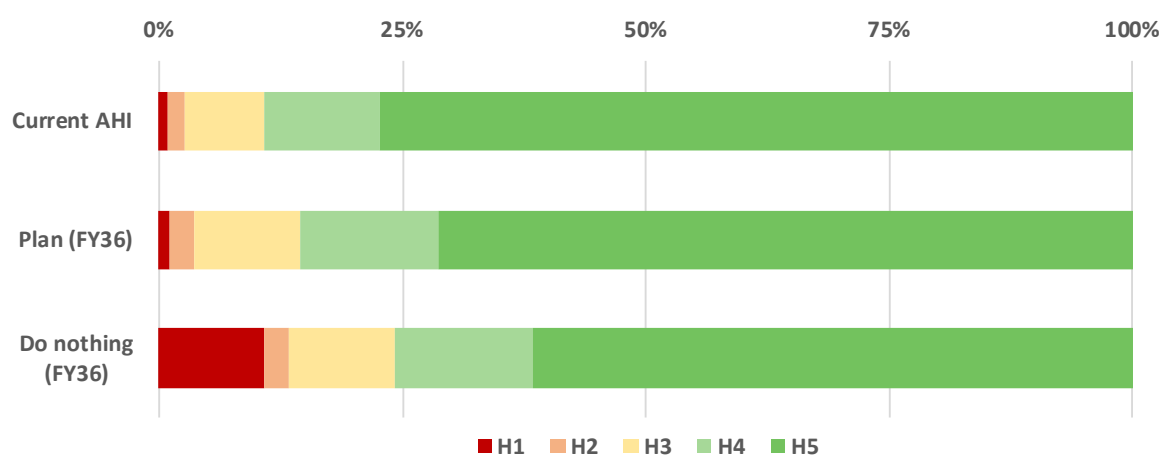
Figure 14.67 Asset health – pole mounted transformers
