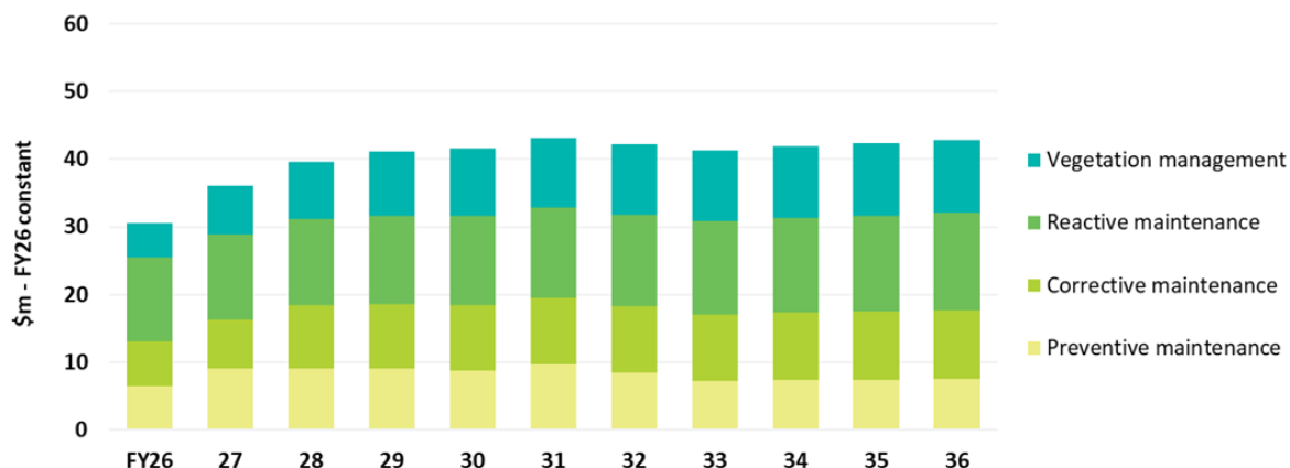
Figure 13.2 Orion's planned total network opex per annum
