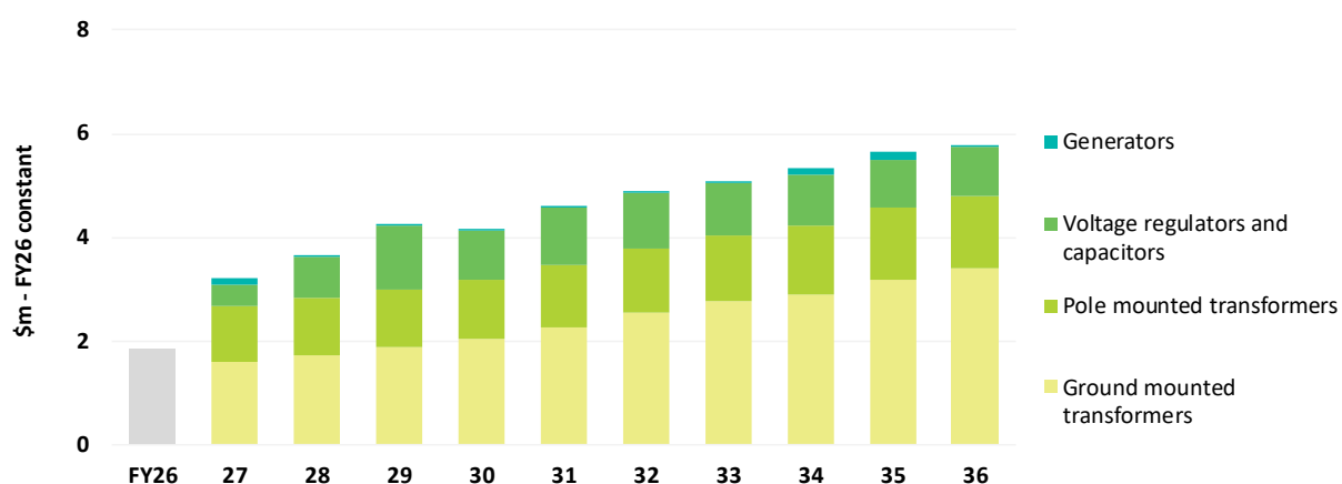
Figure 14.73 Planned distribution transformers renewals capex
