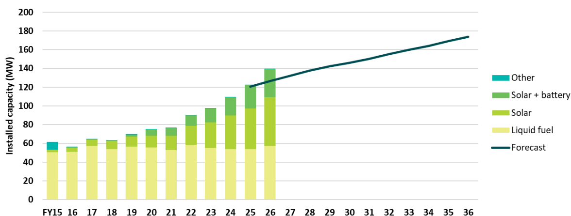
Figure 11.6 Historical and forecast distributed generation on Orion's network, as of 31 March 2026
