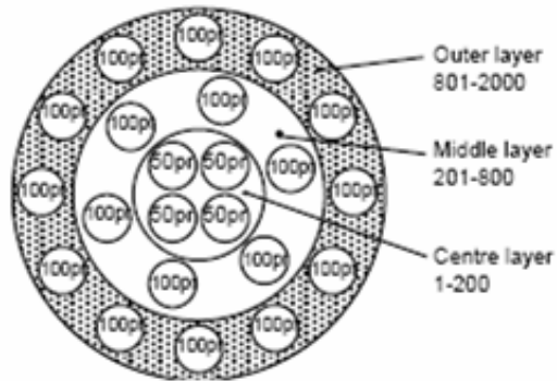
Cross-section of Typical NZ Distribution Cable
