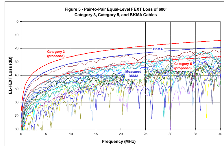
Measured Pair-to-Pair FEXT Losses
