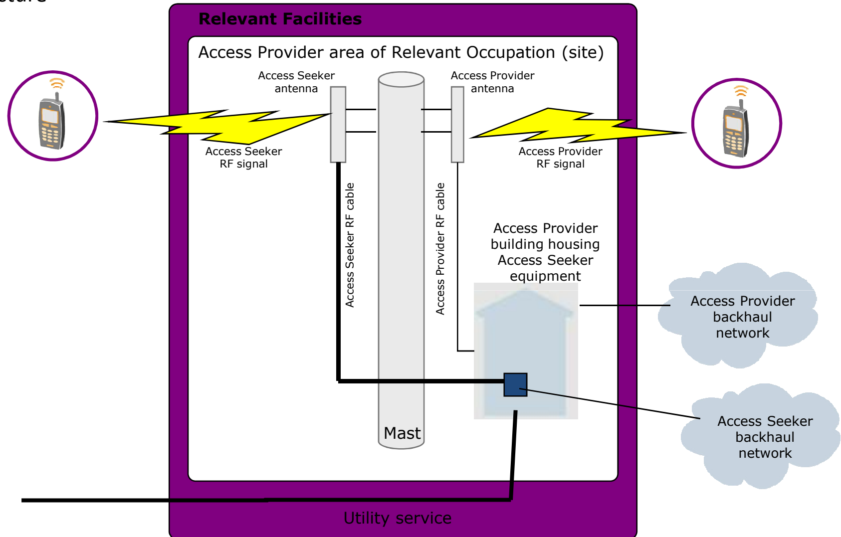
Diagram (b) – Access Seeker equipment housed within Access Provider structure
