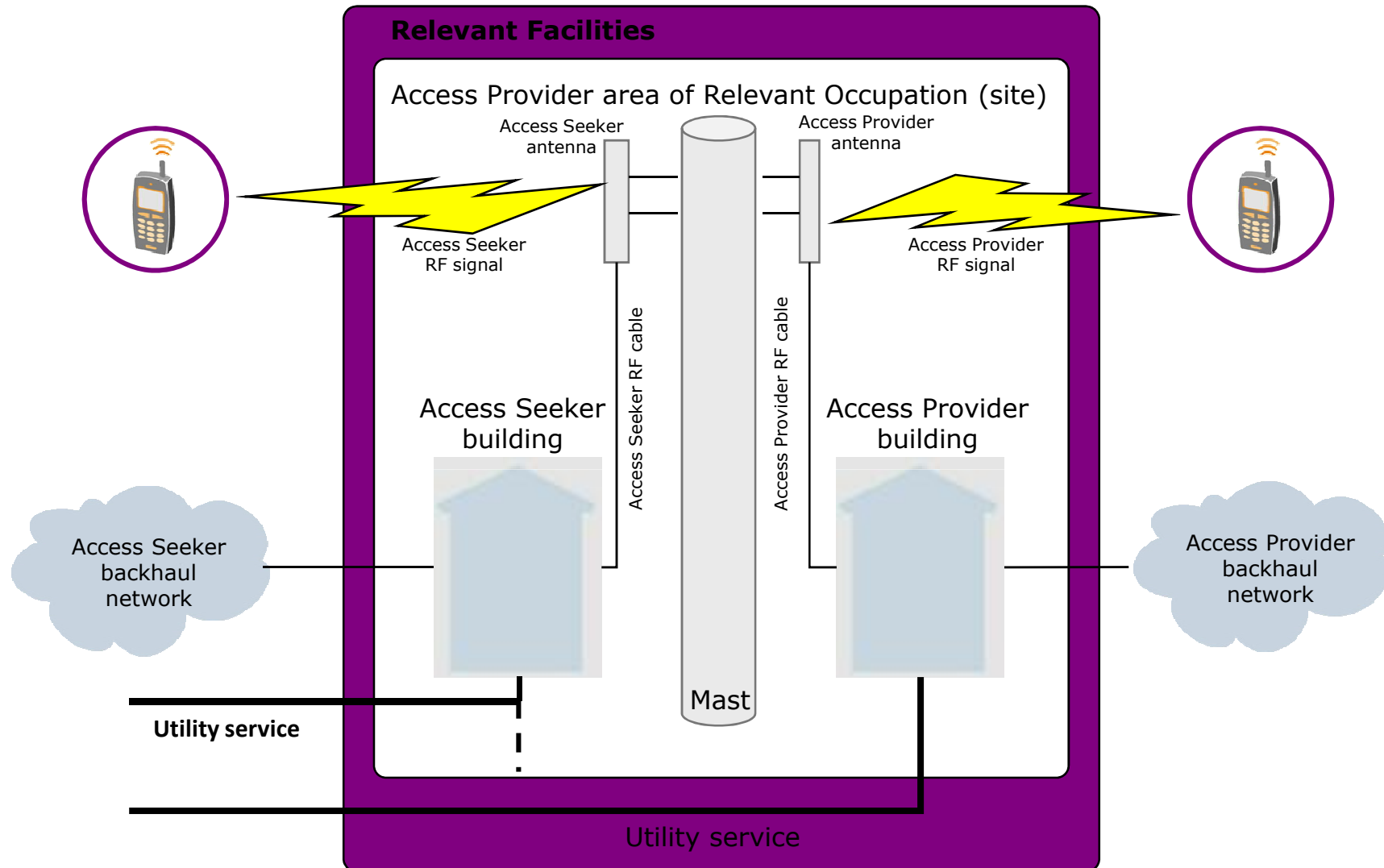
Diagram (a) – Access Seeker uses own utility services
