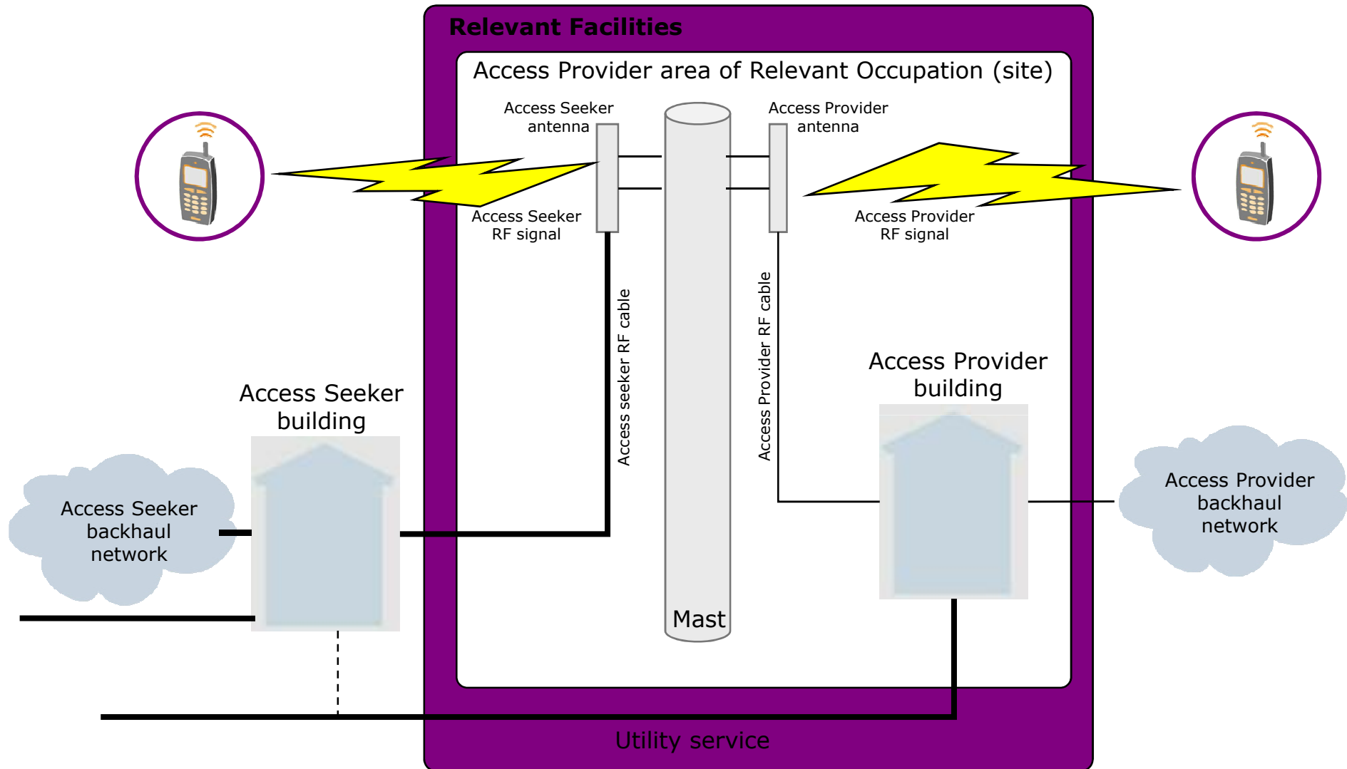
Diagram (c) – Access Seeker building outside of Access Provider site
