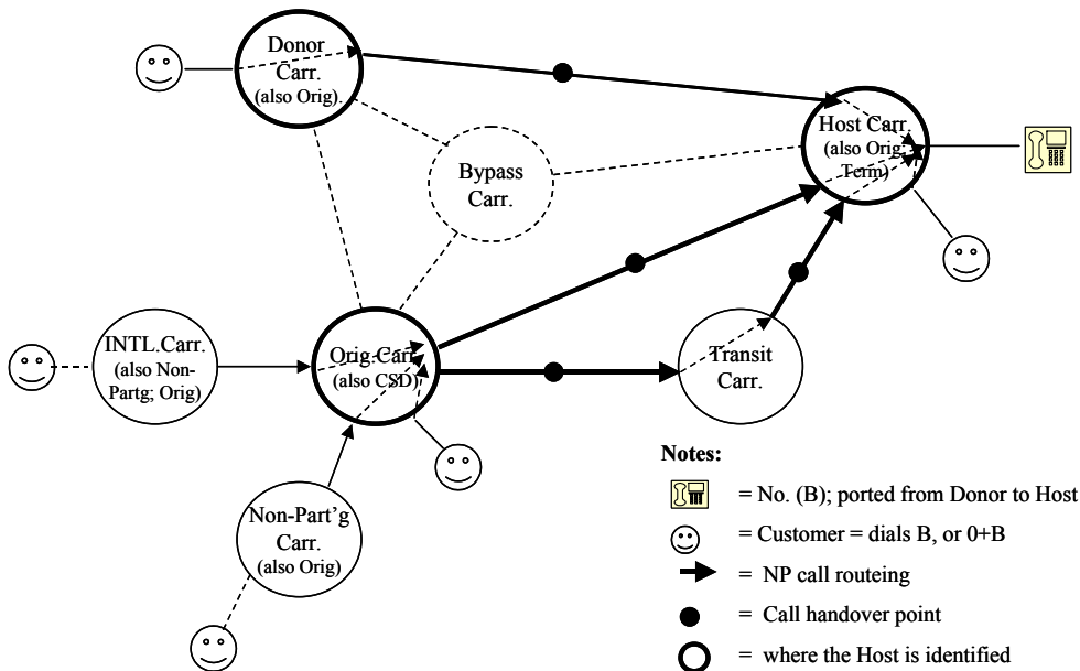
Diagram 2; Orig Carrier Re-Routing (for the initial Port)
